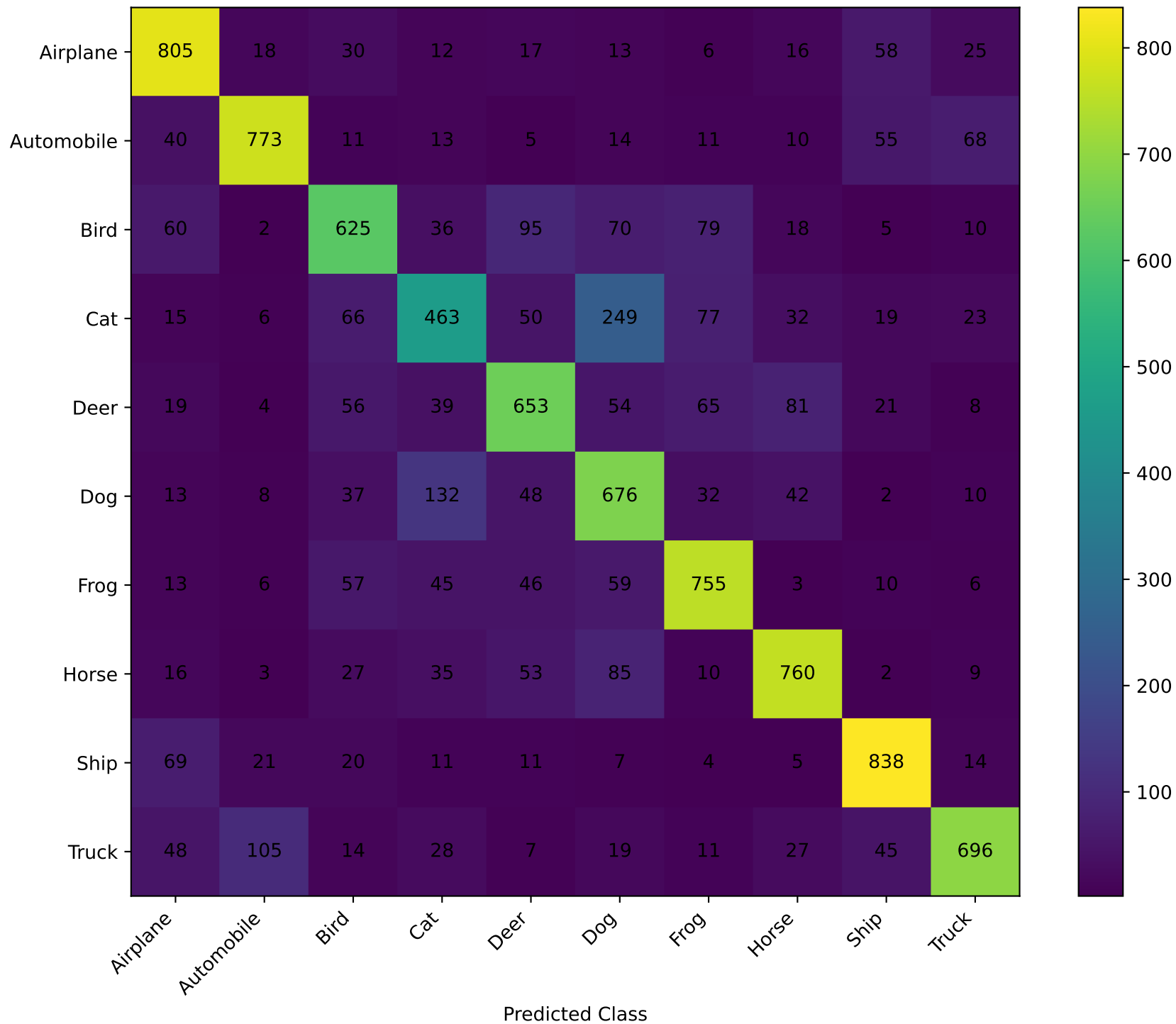
VGG16 Confusion Matrix
